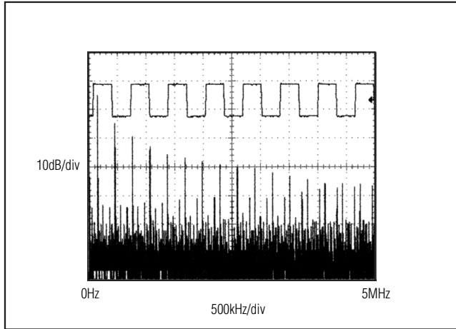
Figure 12. Driver Output Waveform and FFT Plot of MAX481/MAX483/MAX485 Transmitters Transmitting a 150kHz Signal
