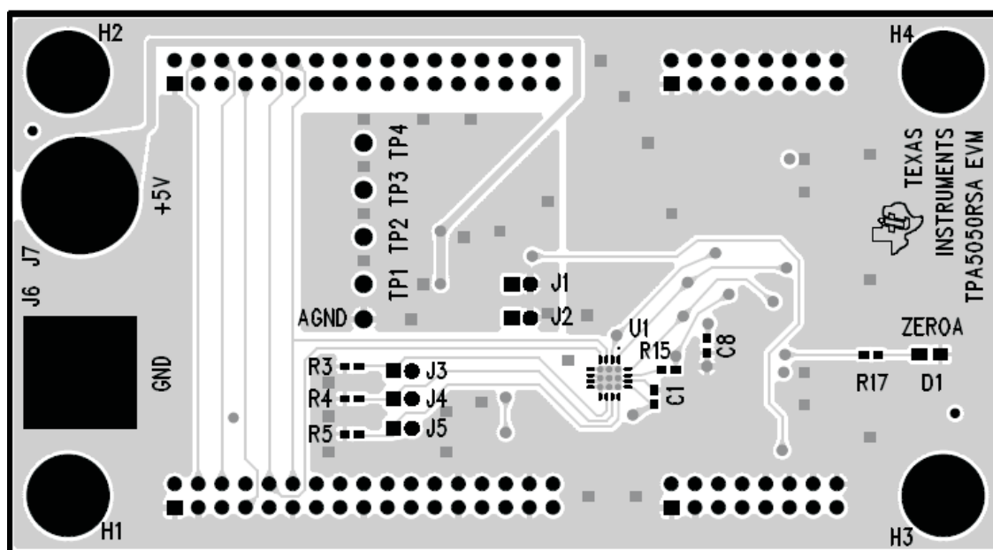
Figure 7. TPA5050EVM Top Layer
