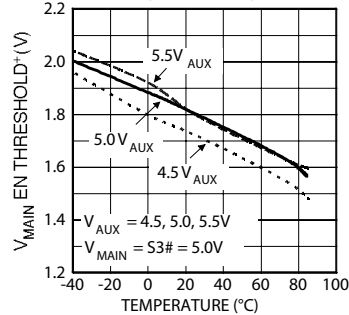
Enable Threshold (increasing) vs. Temperature (MIC2012-1/-2)
