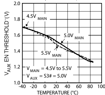
Enable Threshold (decreasing) vs. Temperature (MIC2012-1/-2)
