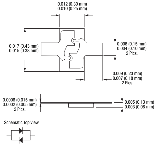
Figure 27. 522-025 Package Dimensions
