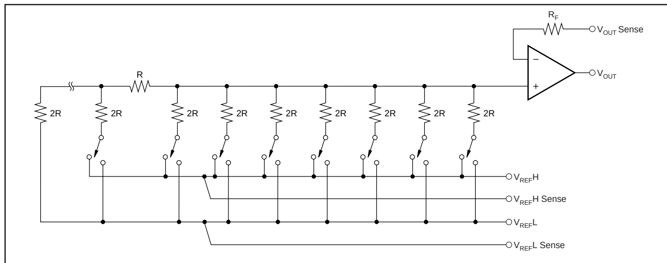
FIGURE 1. DAC7744 Architecture.
