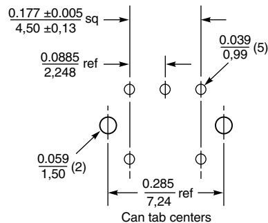
Recommended Board Layout
