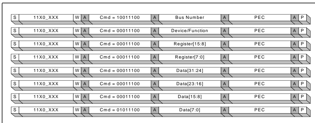
Figure 5-41. SMBus Configuration Write (Write Bytes, PEC Enabled)
