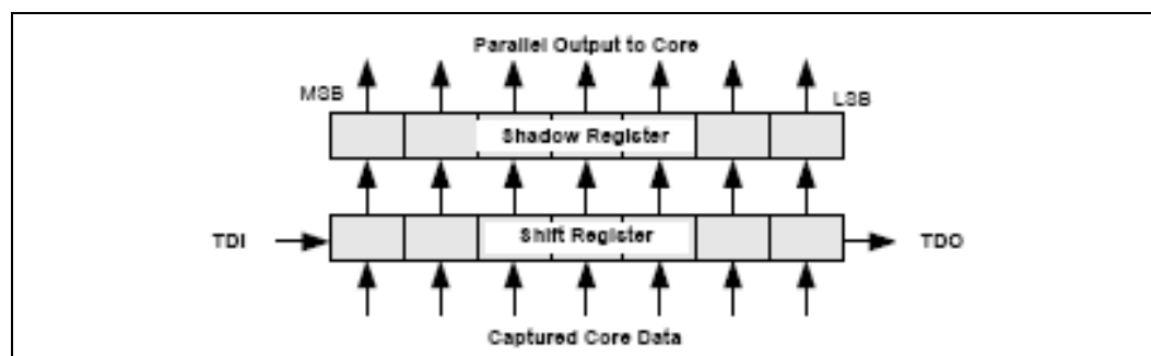
Figure 8-6. TAP Data Register
