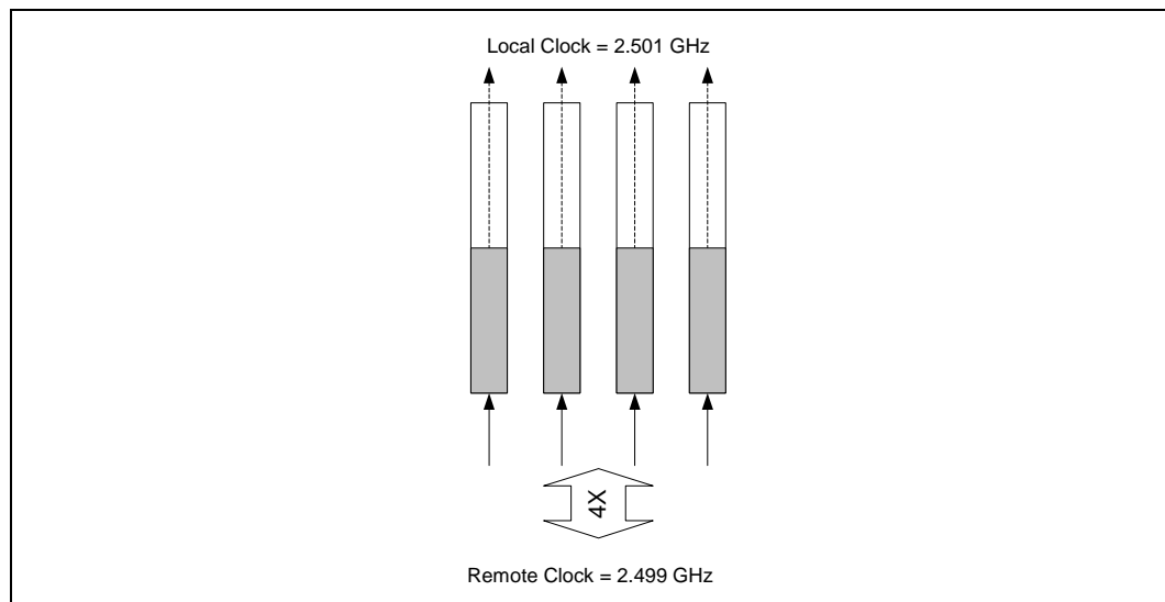
Figure 5-21. PCI Express Elastic Buffer (x4 Example)
