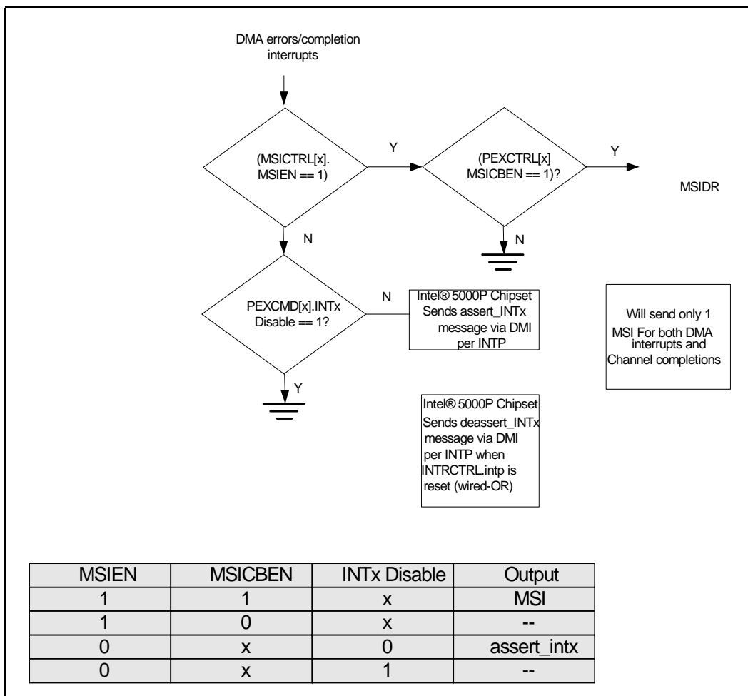
Figure 3-7. Intel 5000P Chipset DMA Error/Channel Completion Interrupt Handling Flow
