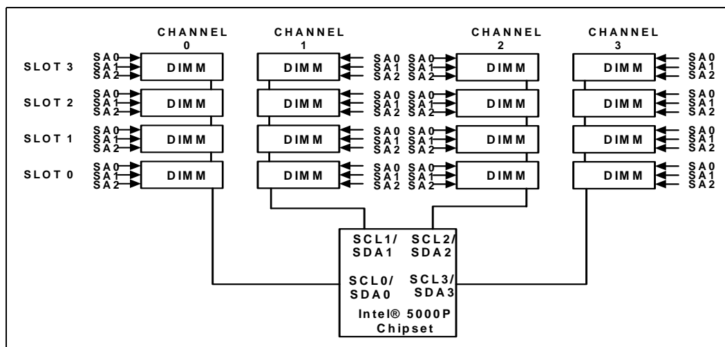
Figure 5-7. Connection of DIMM Serial I/O Signals
