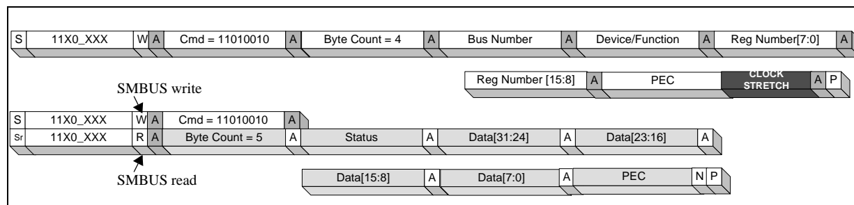
Figure 5-36. SMBus Configuration Read (Block Write / Block Read, PEC Enabled)
