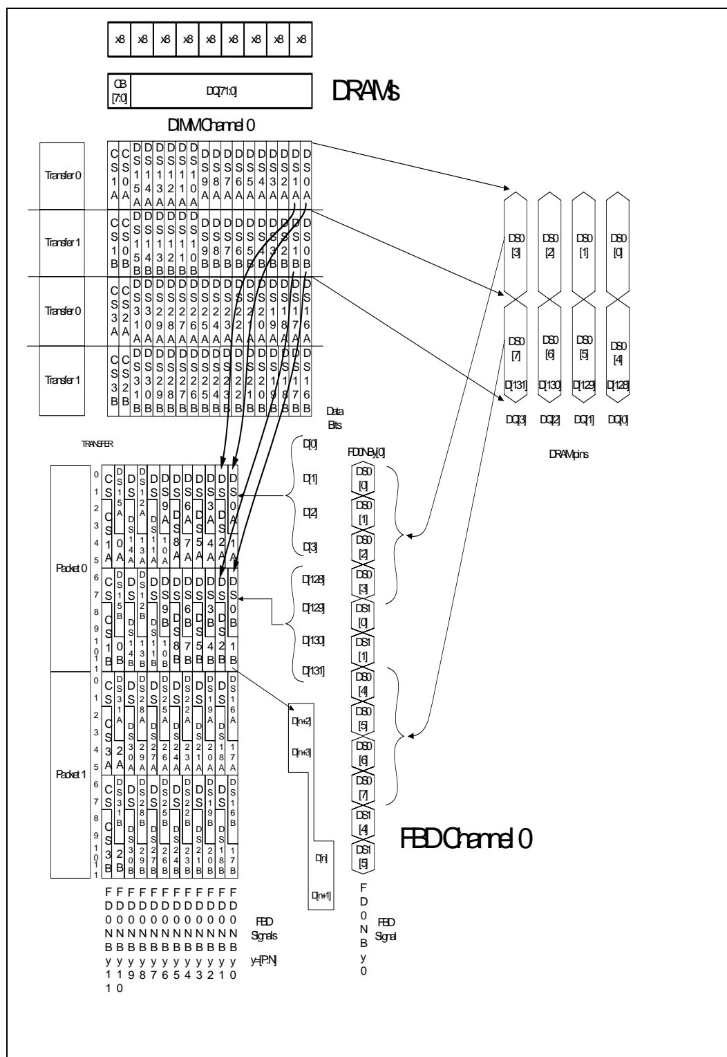
Figure 5-8. Code Layout for Single-Channel Branches
