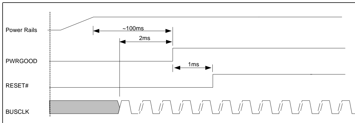
Figure 2-1. Intel 5000P Chipset Clock and Reset Requirements
