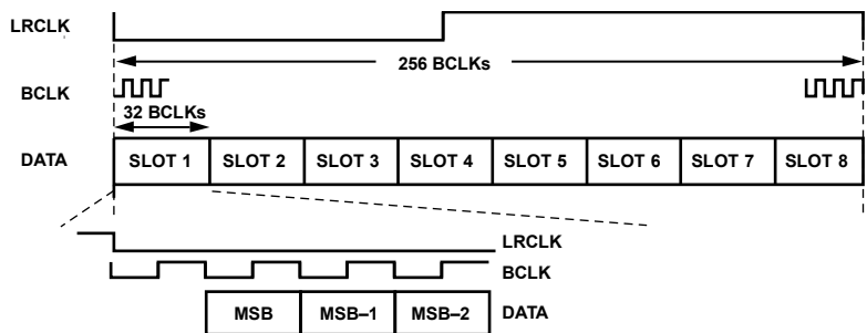
Figure 35. TDM Mode
