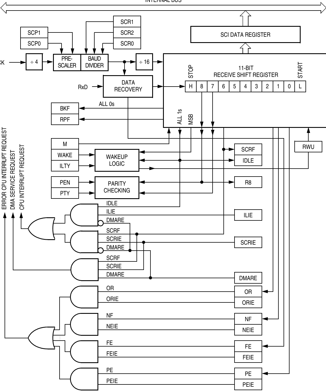
Figure 9-5. SCI Receiver Block Diagram
