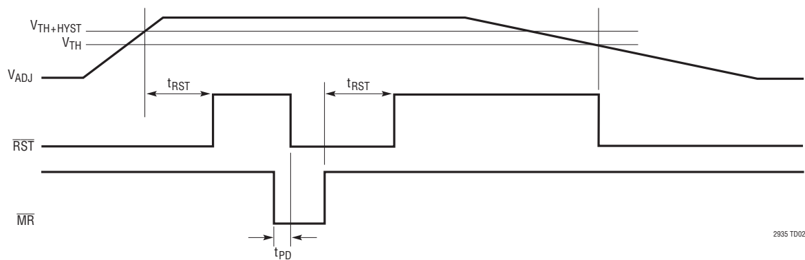
ADJ/RST Timing
