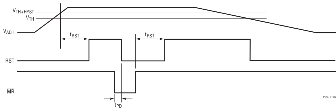
ADJ/RST Timing
