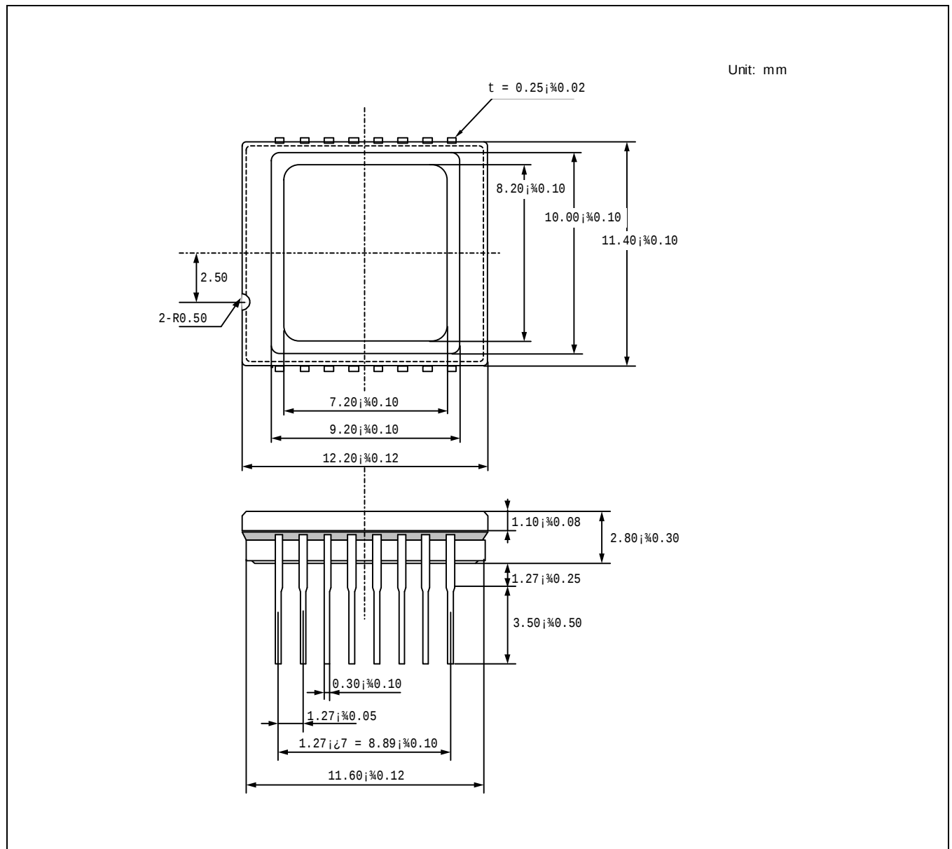
Figure 9. Package Dimensions
