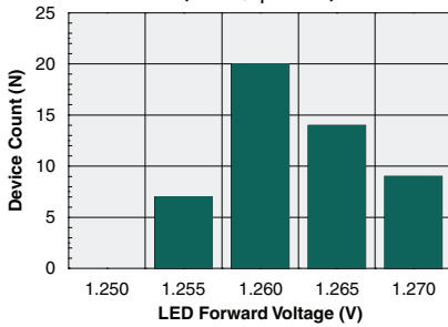
LED Forward Voltage Distribution (N=50, I F =5mA)
