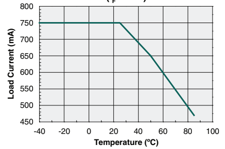
Maximum Load Current vs. Temperature ( I_F=2mA )
