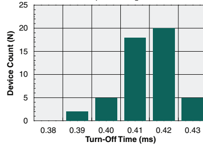
Typical Turn-Off Time Distribution (N=50, I F =5mA, I L =100mA)
