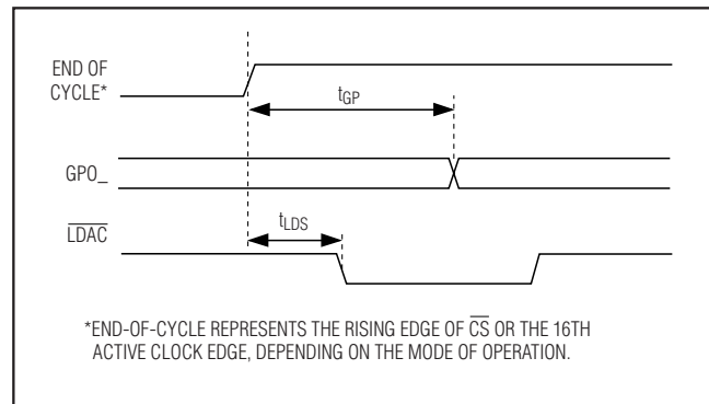
Figure 6. \overline{\text{GPO}} and \overline{\text{LDAC}} Signal Timing
