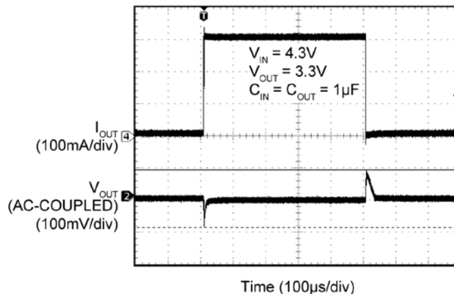
Load Transient
