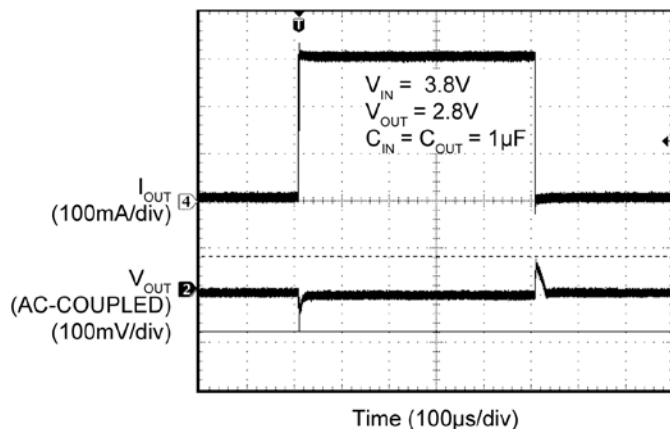
Load Transient
