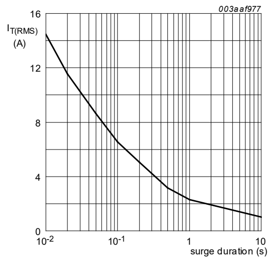
Fig. 2. RMS on-state current as a function of surge duration; maximum values f = 50\text{ Hz} ; T_{lead} = 45\text{ °C}
