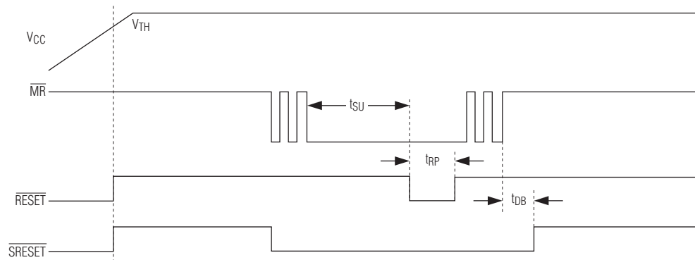
MAX16124/MAX16125; NO RESET TIMEOUT PERIOD AT STARTUP
