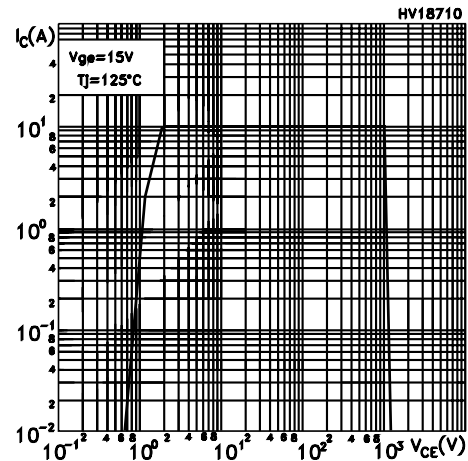
Figure 12. Turn-off SOA
