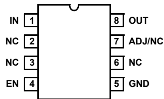
ISL78307 (8 LD EPOIC) TOP VIEW
