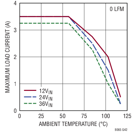
Derating, V_{OUT} = 1.8V , BIAS = 5V, DC2251A Demo Board
