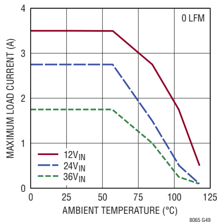
Derating, V_{OUT} = 8\text{V} , BIAS = 5V, DC2251A Demo Board
