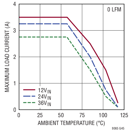
Derating, V_{OUT} = 3.3V , BIAS = 5V, DC2251A Demo Board
