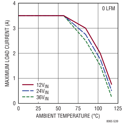
Derating, V_{OUT} = 0.97V BIAS = 5V, DC2251A Demo Board
