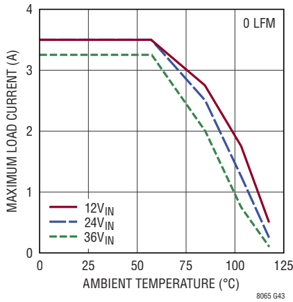
Derating, V_{OUT} = 2V , BIAS = 5V, DC2251A Demo Board
