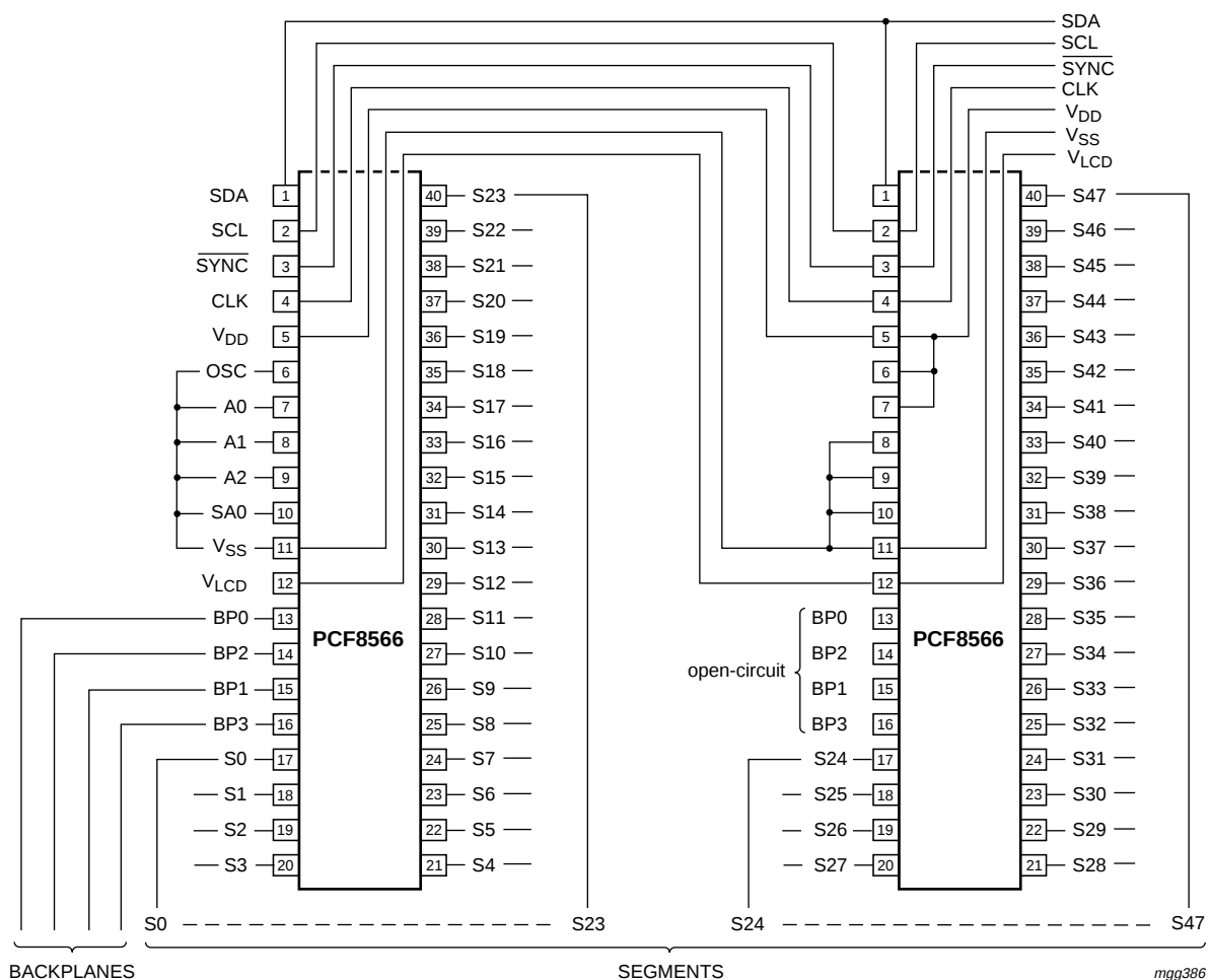
Fig 28. Single plane wiring of packaged PCF8566s
