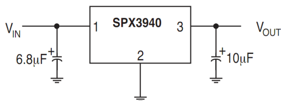
Fig. 20: Fixed Output Linear Regulator
