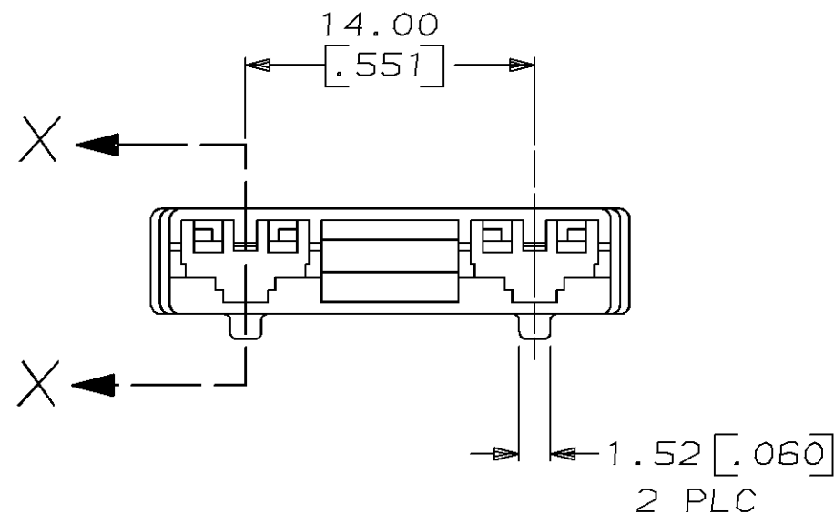
ASSEMBLED VIEW
