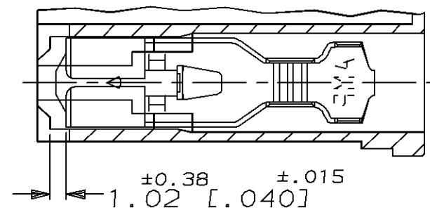
ASSEMBLED VIEW
