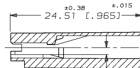
SECTION X-X
