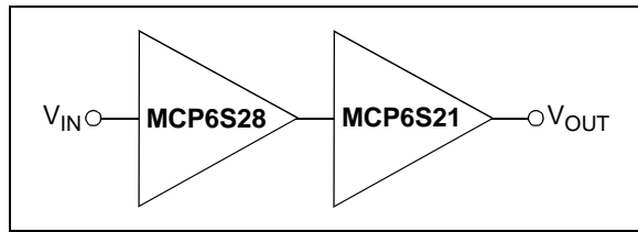
FIGURE 6-6: PGA with Extended Gain Range.
