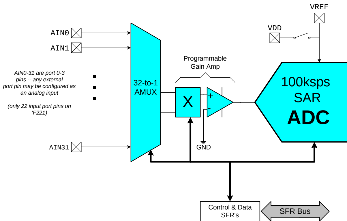
Figure 1.10. ADC Diagram
