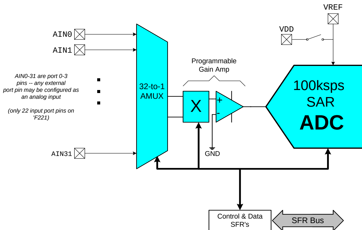
Figure 1.10. ADC Diagram
