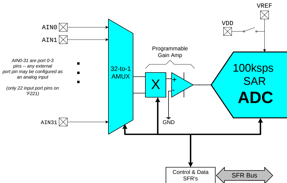
Figure 1.10. ADC Diagram
