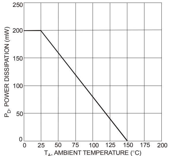
Figure 6 Max Power Dissipation vs. Ambient Temperature
