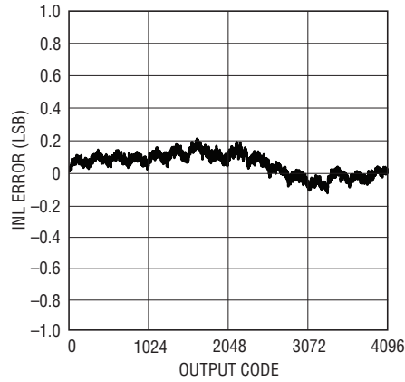
LTC2170-12: Integral Nonlinearity (INL)
