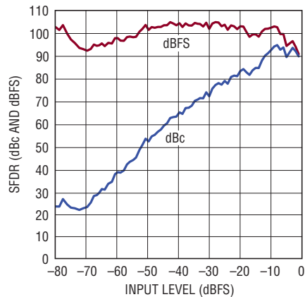
LTC2171-12: SFDR vs Input Level, f_{IN} = 70\text{MHz} , 2V Range, 40Msps
