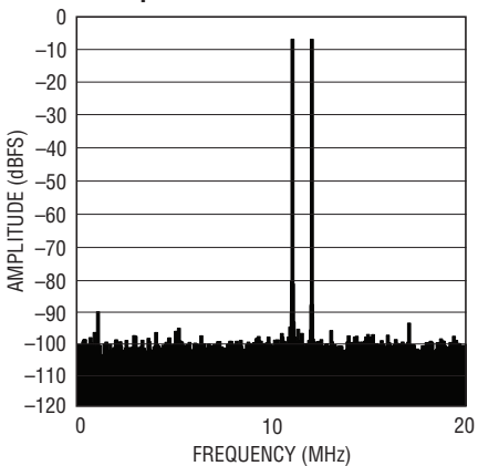
LTC2171-12: 8k Point 2-Tone FFT, f_{IN} = 68\text{MHz}, 69\text{MHz} , -1dBFS, 40Msps
