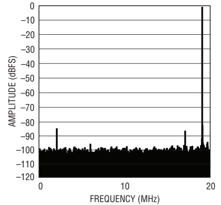
LTC2171-12: 8k Point FFT, f_{IN} = 139\text{MHz} -1dBFS, 40Msps
