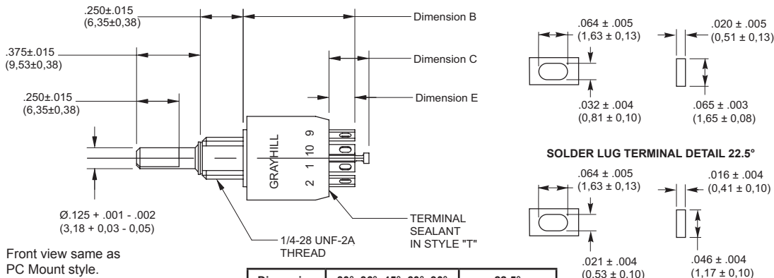
SOLDER LUG TERMINAL DETAIL All angles of throw, except 22.5°
