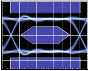
REFERENCE EYE DIAGRAM AT TP1
