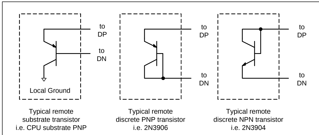
Figure 4.2 Diode Connections
