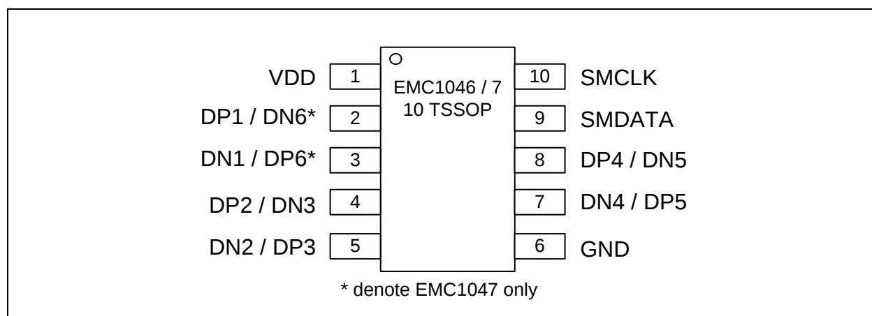
Figure 1.1 EMC1046/EMC1047 Pin Diagram
