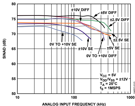
Figure 12. SINAD vs. Analog Input Frequency for Single-Ended (SE) and True Differential Mode (Diff) at 5 V V_{CC}
