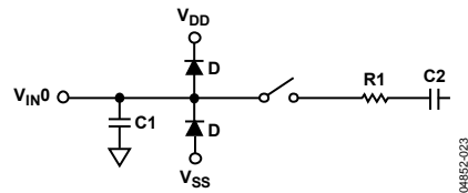
Figure 29. Equivalent Analog Input Circuit, Single-Ended Mode
