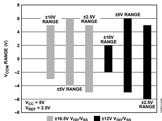
Figure 38. Common-Mode Range for V_{CC} = 5V and V_{REF}/OUT = 2.5V
