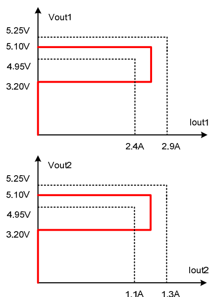
V/I Profile
