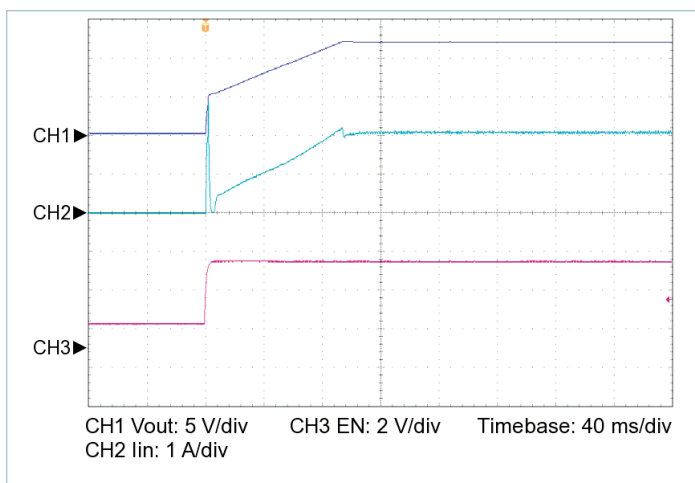
Figure 17 — Startup from EN, V_{IN} = 42\text{ V} , C_{OUT\_EXT} = 10000\text{ μF} , R_{LOAD} = 1.791\text{ Ω}
