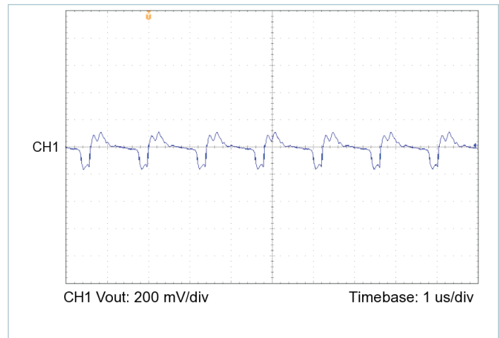
Figure 19 — Output voltage ripple, V_{IN} = 42\text{ V} , V_{OUT} = 12.0\text{ V} , C_{OUT\_EXT} = 1000\text{ μF} , R_{LOAD} = 1.791\text{ Ω}
