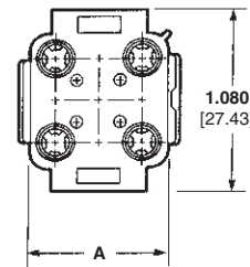
Plug Front
