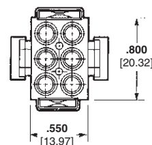
Plug Front
