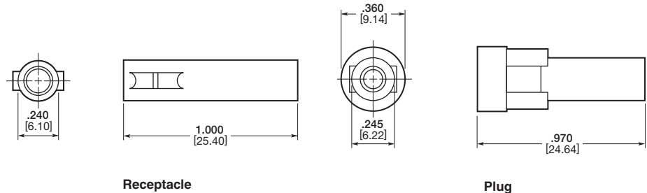
Plug
