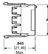
Cap Rear
