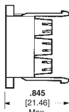
Plug Rear
