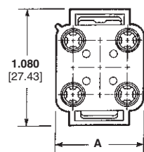
Plug Rear
