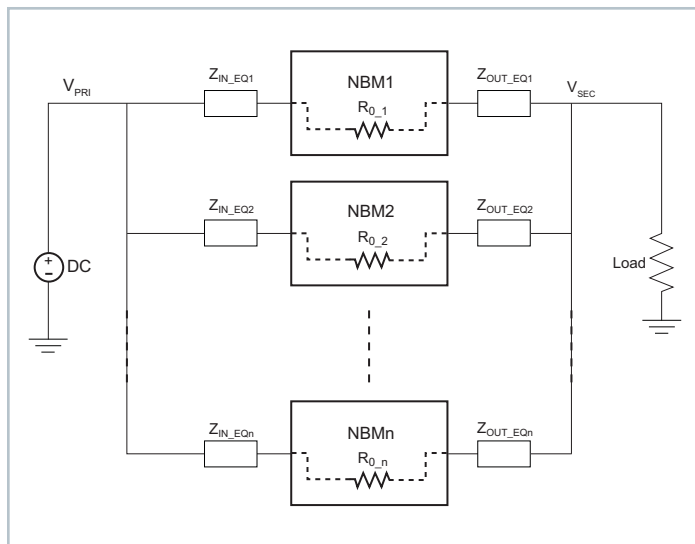
Figure 22 — NBM module array
