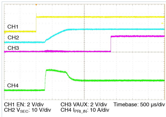
Figure 15 — Start up from application of EN with pre-applied V_{PRI\_DC} = 42 V, 20% I_{SEC\_DG} , 100% C_{SEC\_OUT\_EXT}
