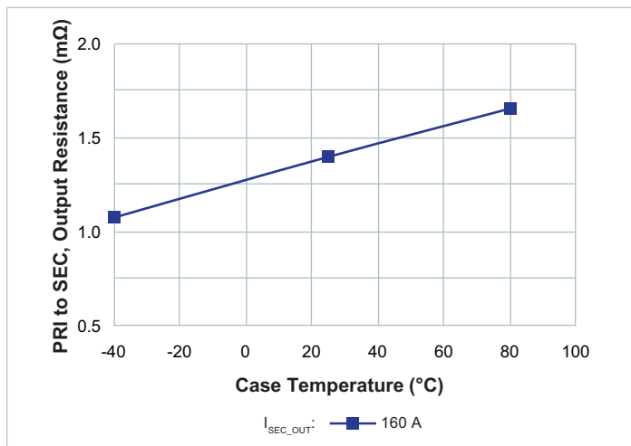
Figure 9 — R_{OUT} vs. temperature; Nominal V_{PRI\_DC} I_{SEC\_DC} = 160 A at T_{CASE} = 80^\circ C
