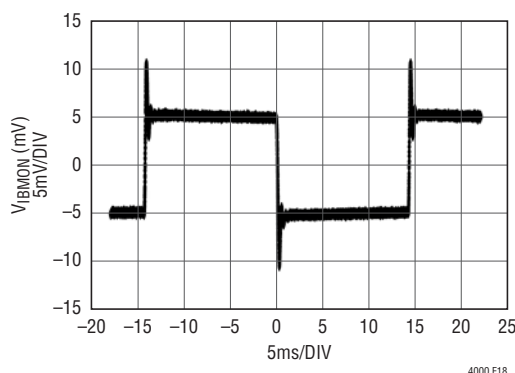
Figure 18. Transient Response of Charge Current Regulation Loop Observed at IBMON When V_{\text{OFB}} is Regulated to V_{\text{OUT(INST\_ON)}} with C_C = 22\text{nF} , R_C = 20\text{k} for a 100\text{mA} Charge Current Step
