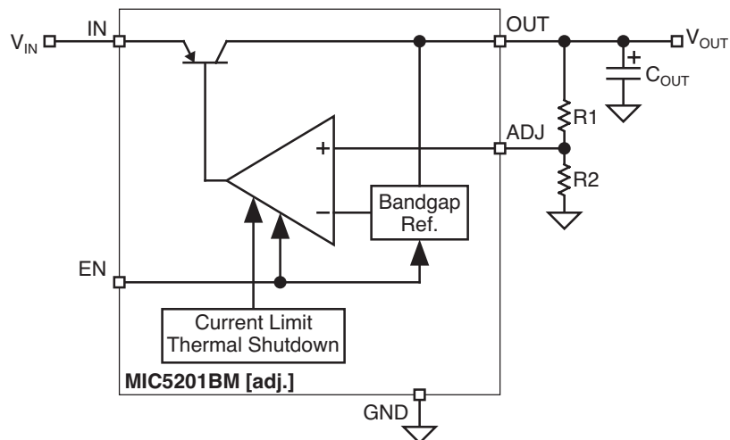
Adjustable Regulator
