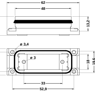
Dimensions: Panel mounting frame
