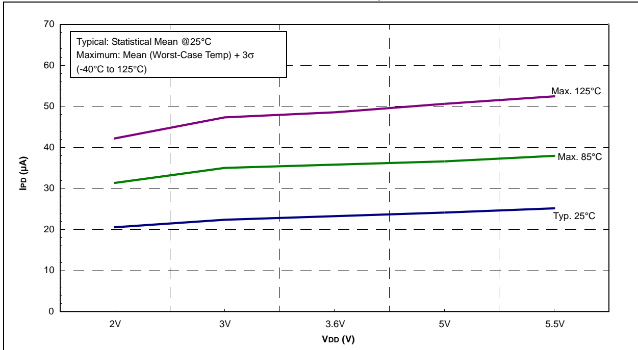
FIGURE 24-33: PIC16F72X BOR I PD vs. V DD , V CAP = 0.1μF
