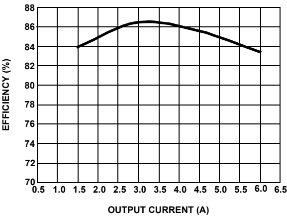
FIGURE 8. MEASURED EFFICIENCY V_{IN} = 12\text{V} , V_{OUT} = 3.3\text{V}
