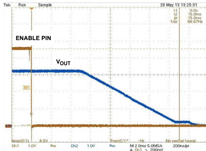
FIGURE 13. RAMP-DOWN TIME SETTING OF 5ms Delay, 10ms FALL
