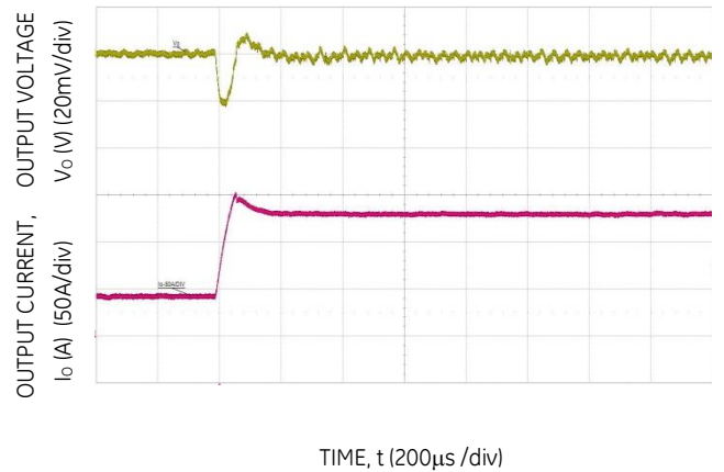
Figure 16. Transient Response to Dynamic Load Change from 25% to 75% at 12Vin, C_o = 12 \times 47\mu\text{F} + 10 \times 1000\mu\text{F} , R_{TUNE} = 3.01\text{k}\Omega .
