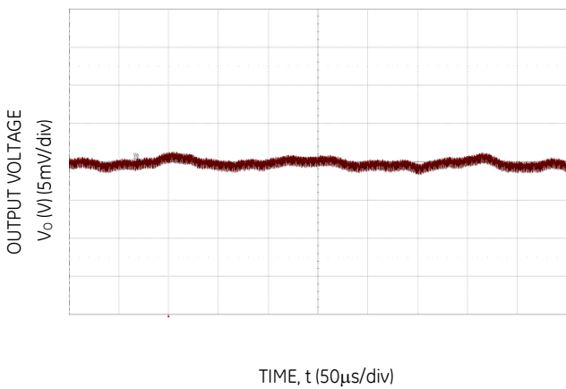
Figure 3. Typical output ripple and noise (C o =12x47μF ceramic + 10x470μF polymer, V IN = 12V, I o = I o,max ).
