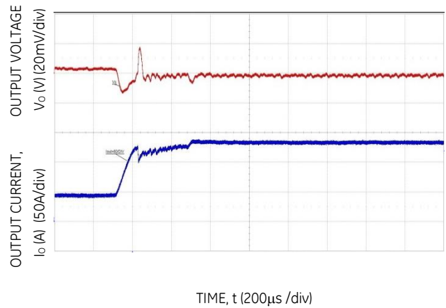
Figure 4. Transient Response to Dynamic Load Change from 25% to 75% at 12V in , C o = 12 x 47μF + 10 x 1000μF, R TUNE = 3.01kΩ.
