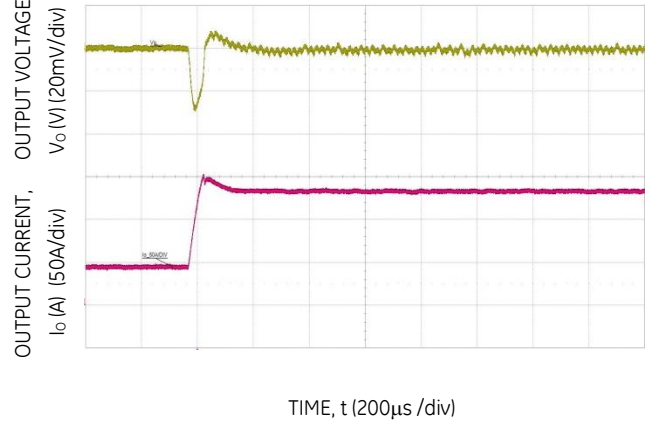
Figure 22. Transient Response to Dynamic Load Change from 25% to 75% at 12Vin, C o = 12 x 47µF + 10 x 1000µF, R TUNE = 3.01kΩ.
