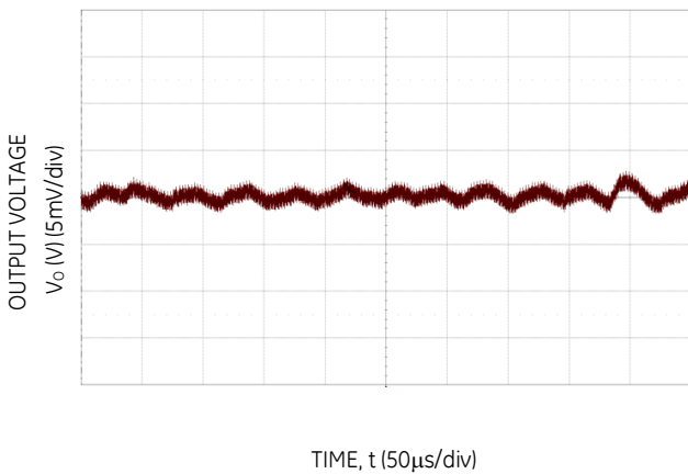
Figure 27. Typical output ripple and noise ( C_0=12 \times 47\mu\text{F} ceramic + 10 \times 470\mu\text{F} polymer, V_{IN} = 12\text{V} , I_o = I_{o,max} )
