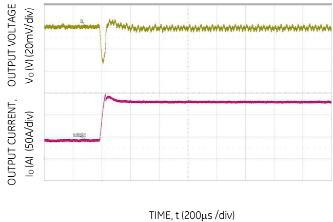
Figure 28. Transient Response to Dynamic Load Change from 25% to 75% at 12Vin, C_0 = 12 \times 47\mu\text{F} + 10 \times 1000\mu\text{F} , R_{TUNE} = 3.01\text{k}\Omega .
