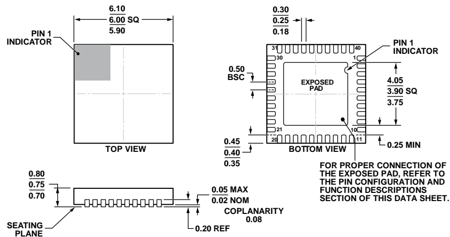
COMPLIANT TO JEDEC STANDARDS MO-220-WJJD. Figure 75. 40-Lead Lead Frame Chip Scale Package [LFCSP_WQ] 6 mm × 6 mm Body, Very Very Thin Quad (CP-40-14) Dimensions shown in millimeters
