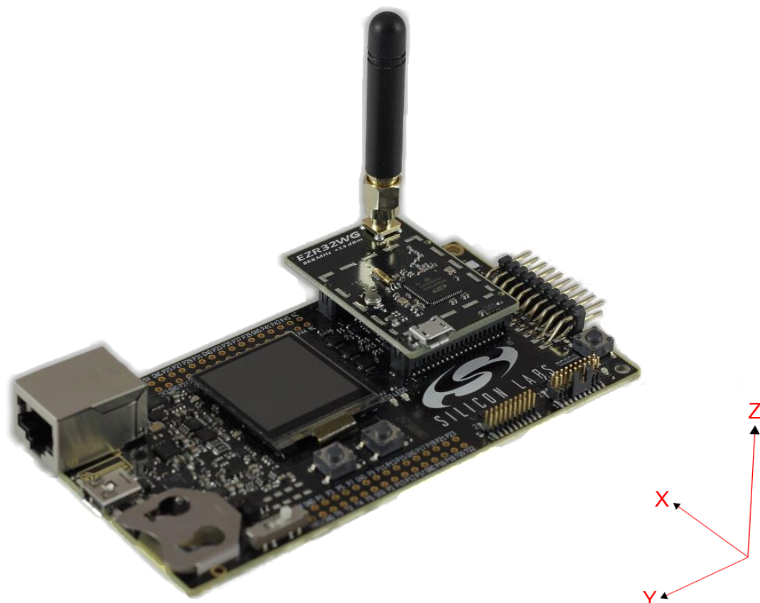
Figure 6.2. DUT: BRD4502A (Rev. B00) Radio Board with Wireless Starter Kit Mainboard
