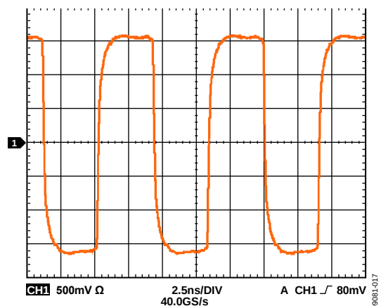
Figure 14. Output Waveform (Differential), HSTL at 16 mA, 122.88 MHz
