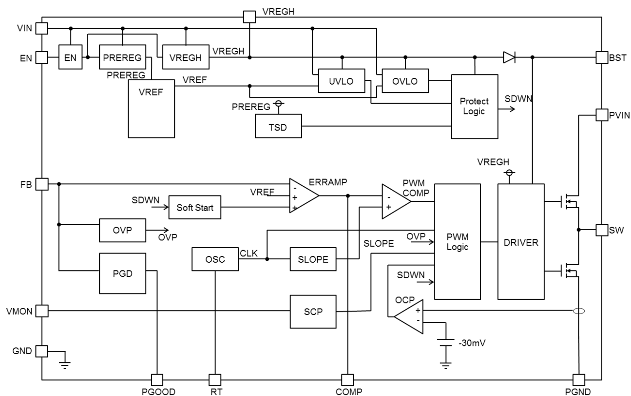
Figure 3. Block Diagram
