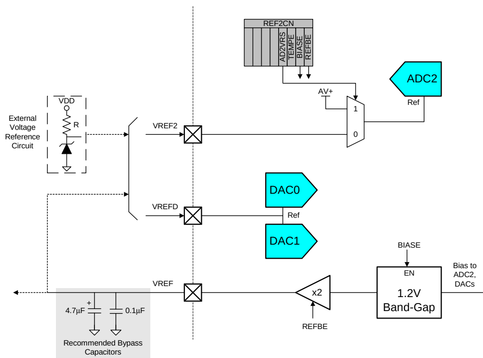
Figure 9.1. Voltage Reference Functional Block Diagram
